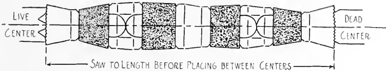
FIG. 540. METHOD OF TURNING CORE-PRINTS.
